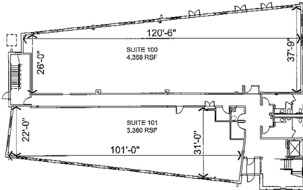
1 1 FLOOR PLAN FIRST FLOOR
