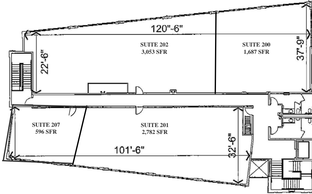
2 1 FLOOR PLAN SECOND FLOOR
